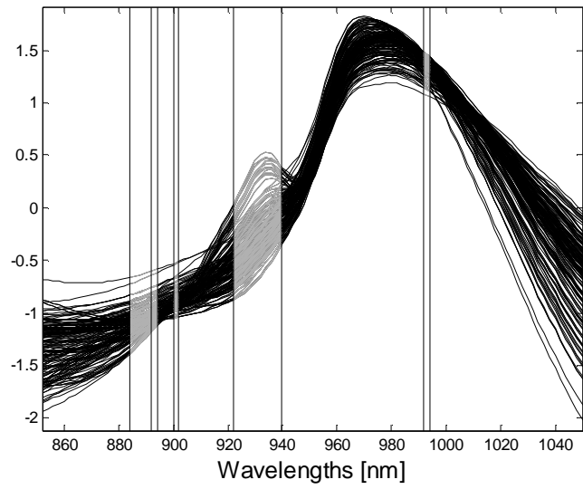
Figure 3: Tecator spectra and spectral variables selected by the clustering approach (in grey).
