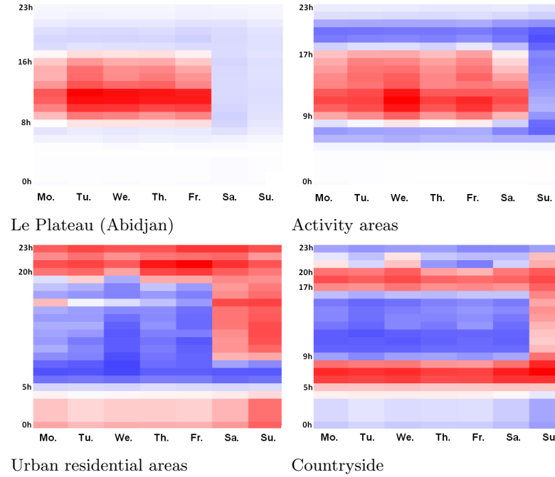
Fig. 7. Calendars of excesses (red) and lacks of calls emitted from each of the four clusters of antennas, in function of the weekday and the daytime.
